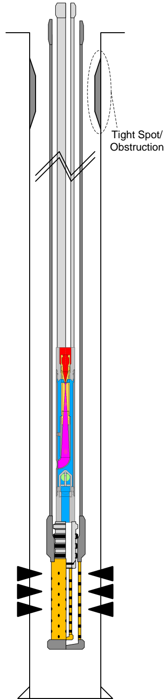
SLIM HOLE
